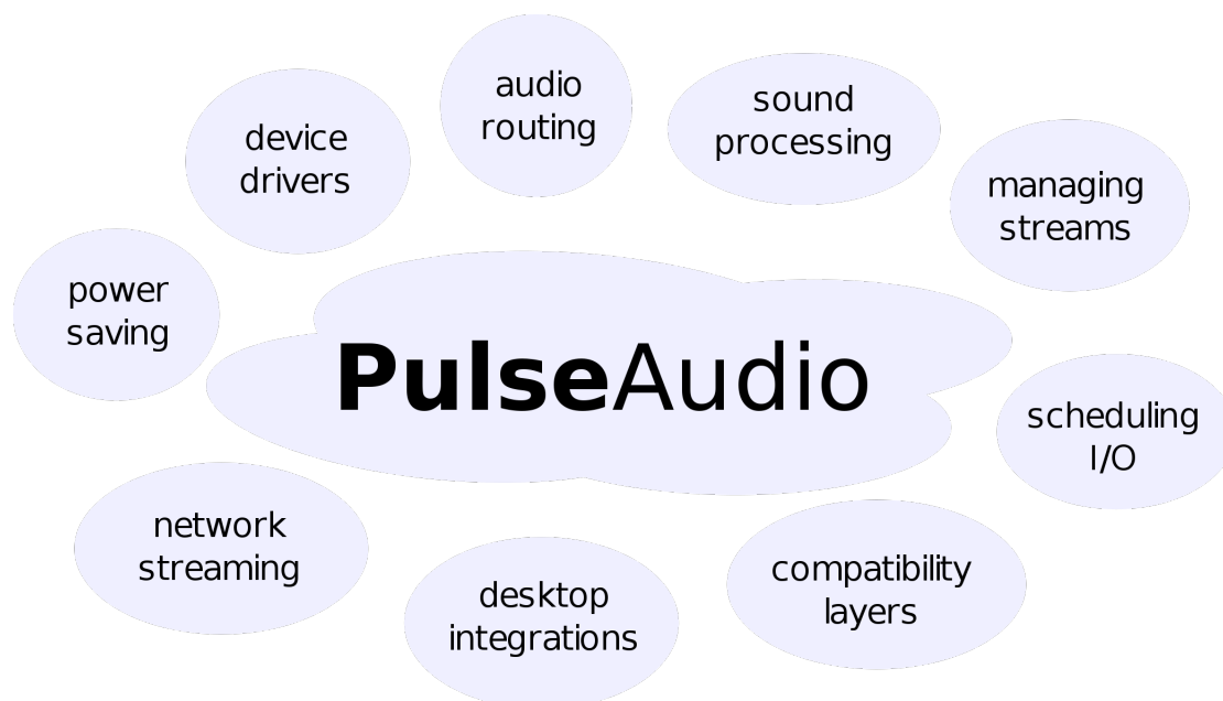
Figura 15 – Pulseaudio
